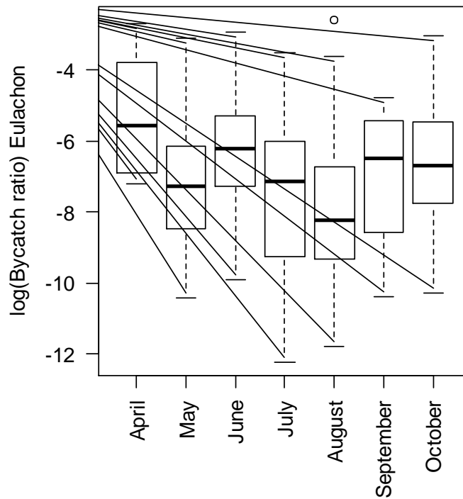
Figure 17. Boxplots of the natural logarithm of the bycatch ratio of eulachon for month fished in 2011.
