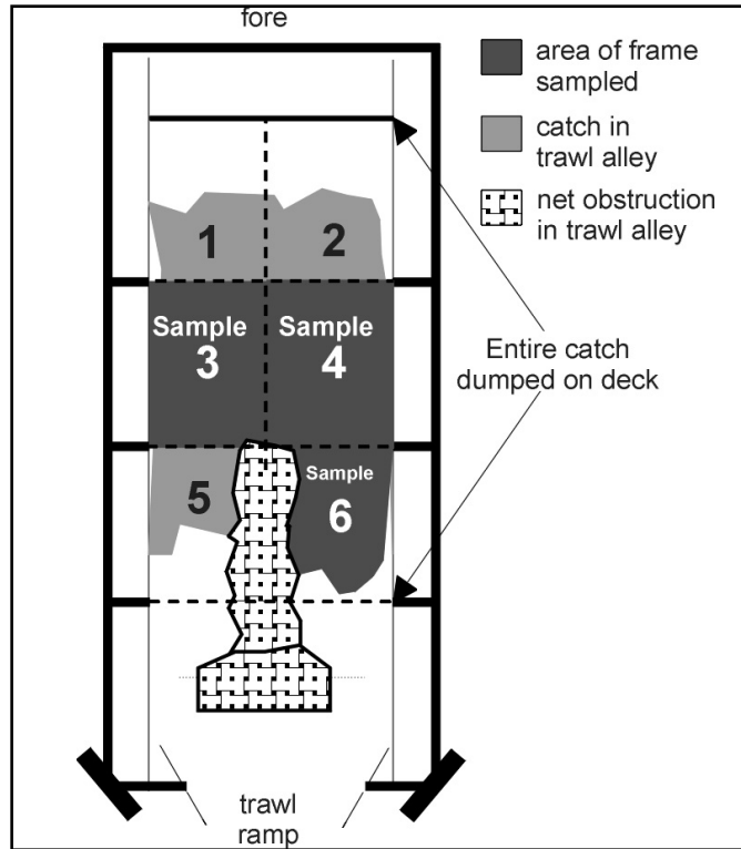
Figure 5-1: Spatial Design Using Trawl Alley
