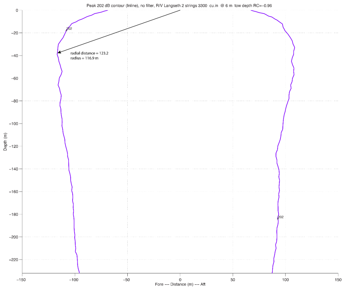
FIGURE A-8. Modeled deep-water received Peak SPL from the 18-airgun array at a 6-m tow depth. The plot provides the distance to the 202-dB Peak isopleth.
