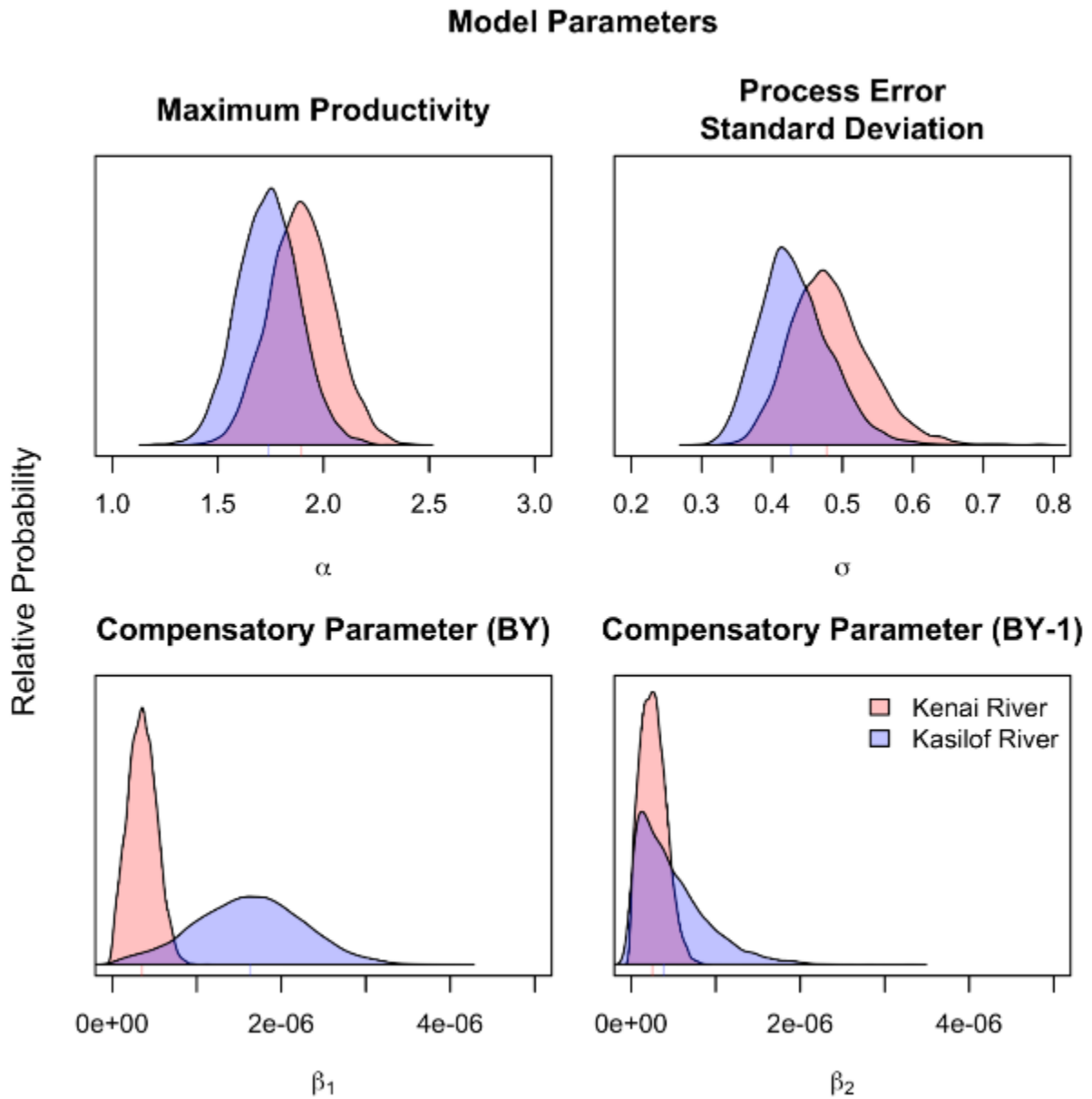
Figure 8. Posterior distributions for brood year interaction Ricker model parameters. The highest point on each distribution indicates the parameter value with the highest posterior probability density given the data. Vertical lines on the x-axis highlight the posterior median parameter value for each population.
