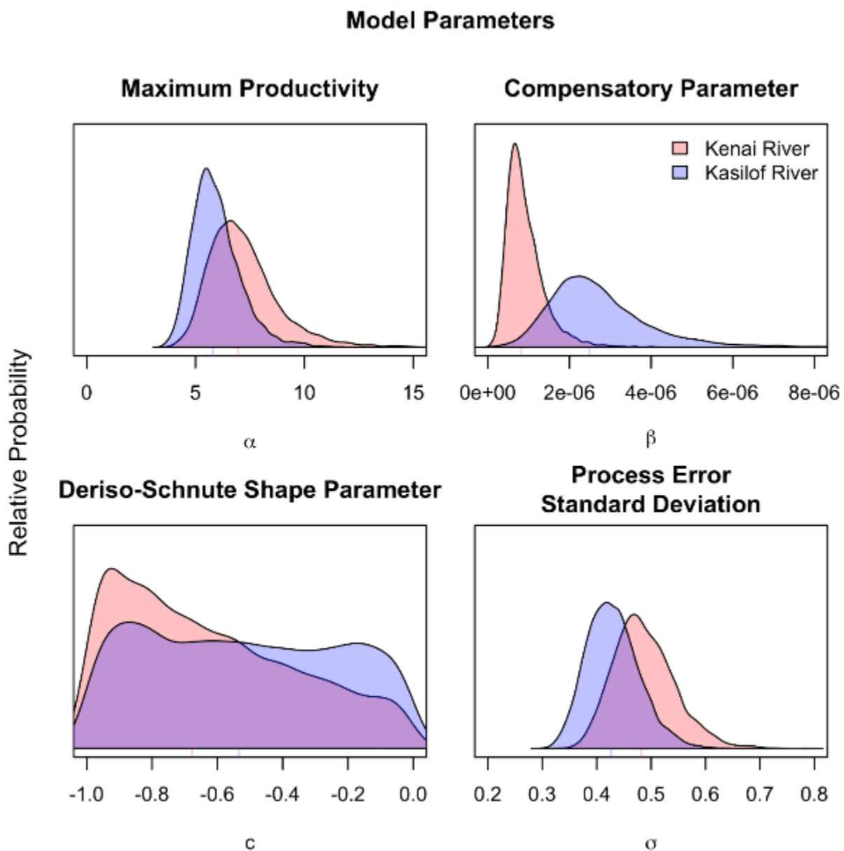
Figure 14. Posterior distributions for Deriso-Schnute model parameters. The highest point on each distribution indicates the parameter value with the highest posterior probability density given the data. Vertical lines on the x-axis highlight the posterior median parameter value for each population.
