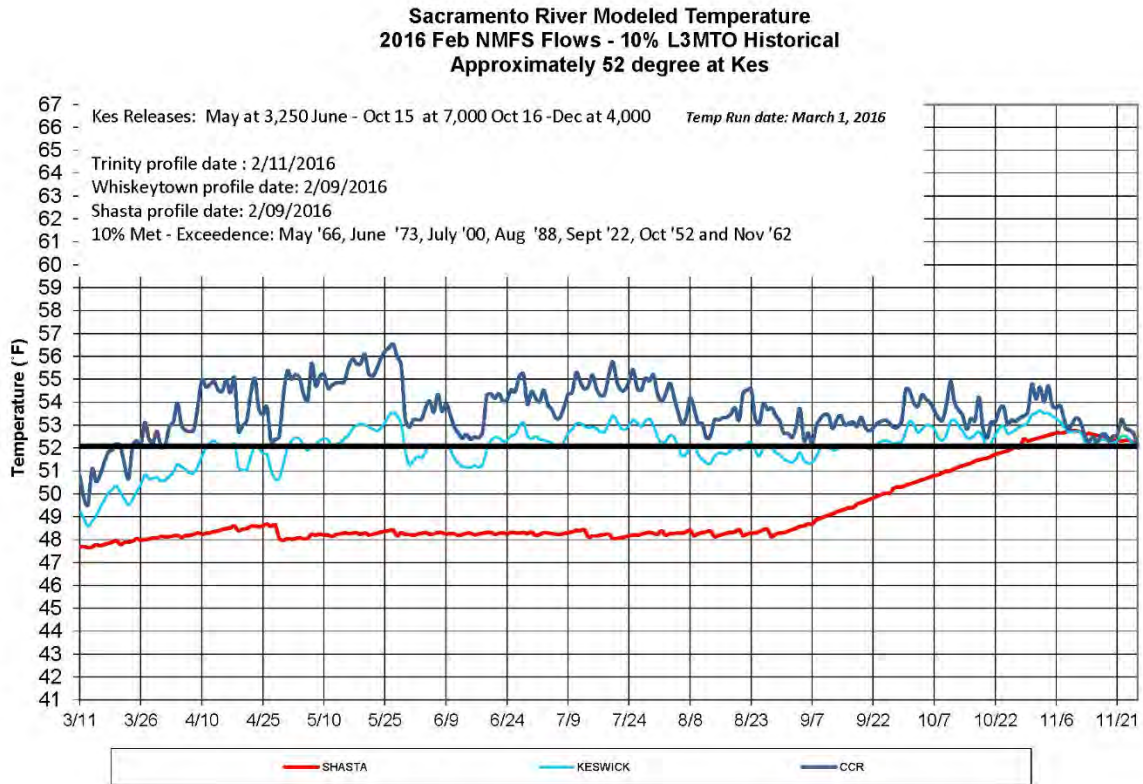
Figure 7. Reclamation’s Sacramento River Modeled Temperature Results using the 2016 February 90% exceedance outlook, historical 10% local 3-month temperature outlook meteorology, NMFS-scenario for Keswick Dam monthly average releases for May through November, and targeting approximately 52°F DAT at KWK.
